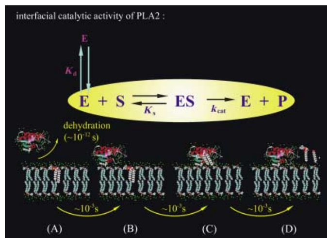
Figure 4. Reaction pathways in the catalytic activity of the protein PLA2. K_d indicates the equilibrium dissociation constant of the enzyme to the membrane. K_s and k_{cat} denote the equilibrium dissociation of the enzyme-substrate complex and catalytic rate constant (see text). Schematic representation of the catalytic steps of the enzyme: A) The enzyme and the host that contains the substrate. B) The complex of the enzyme with the host. C) The complex of the enzyme with the membrane-bound substrate. D) The products. The timescales represent an estimate for the different processes involved. [2]
